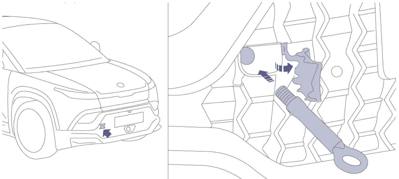
Front attachment point
